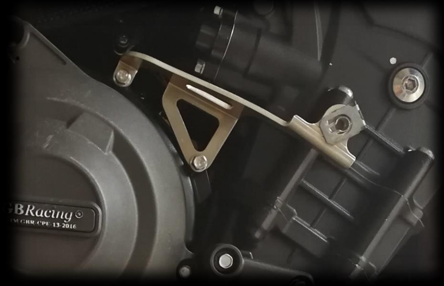
upper bracket right Daytona 2006 till 2012 & any Street Triple
